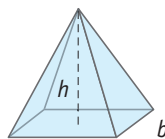
piramide retta
